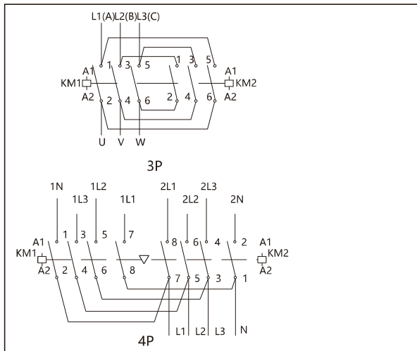
Connection of connection plate
